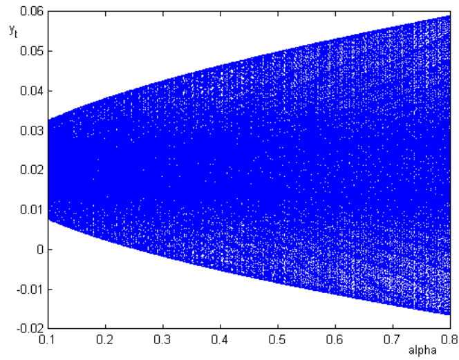
Figure 8: Bifurcation diagram when \alpha is varied
