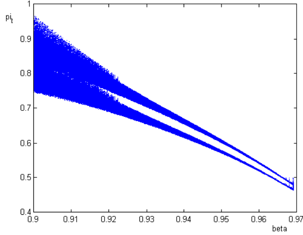
Figure 4: Bifurcation diagram for \beta
