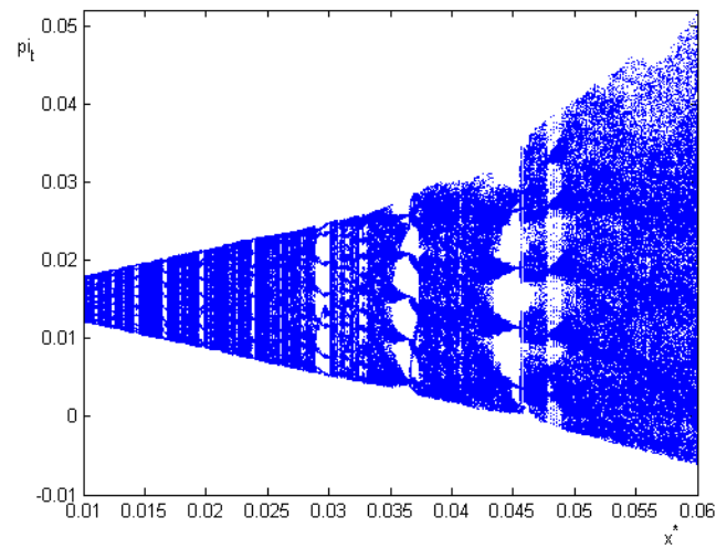
Figure 10: Strange attractor for the inflation rate produced when the target value for the output gap is changed..
