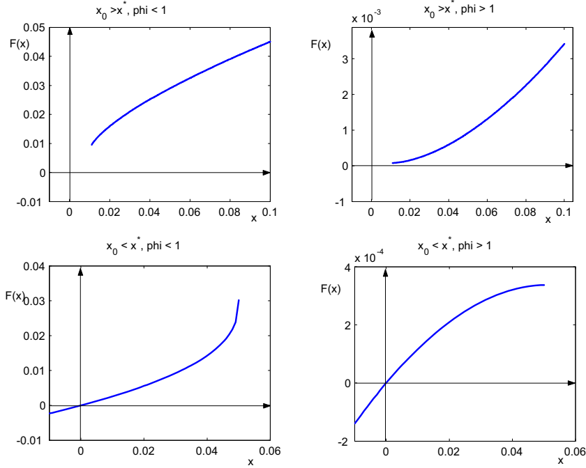
Figure 3: The nonlinear Phillips curve
