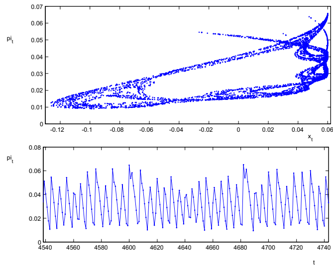
Figure 13: Strange attractor and time series of \pi_t
